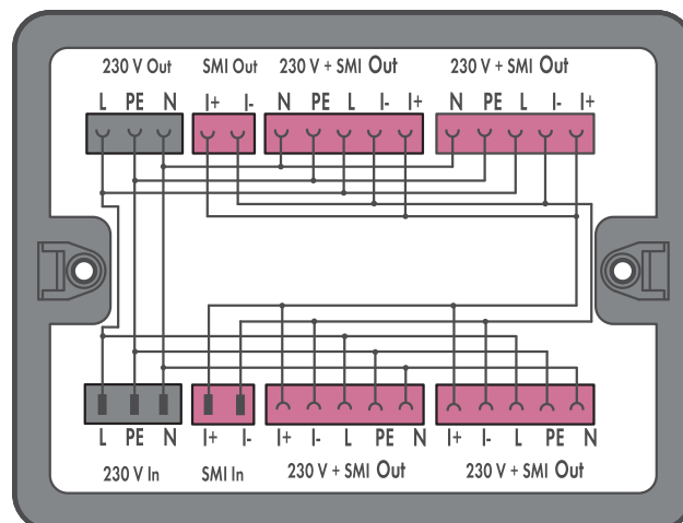
Distribution box; 230 V + SMI
